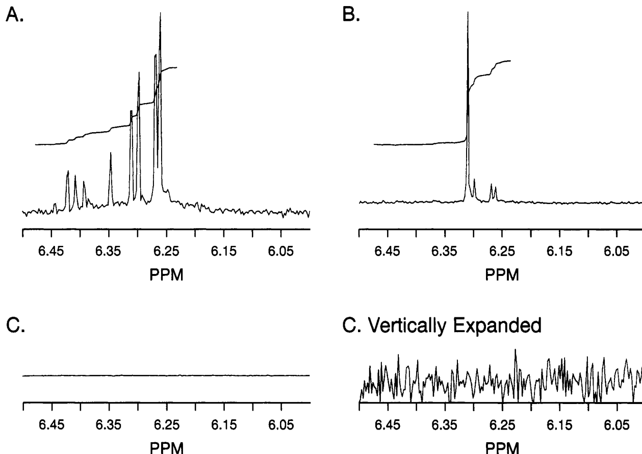
Figure 1. (A and B) Expanded 1 H NMR of vinyl region of the reaction of methyl iodide with the precipitated thiolate salts of 3, 4, 5, and 6, as prepared via literature method (see Experimental Section, reaction 3, runs 1 and 2, pathway B, with precipitation). Spectra A and B demonstrate the variability of the reaction. (C) Expanded 1 H NMR of vinyl region of a reaction of methyl iodide with 2 as prepared via new method. (C vertically expanded) Same vinyl region as (C), expanded vertically 60X.
