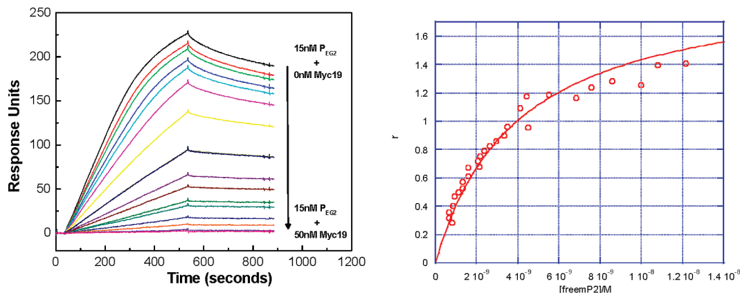
Figure 5. SPR analysis of P_{\text{egg2}} binding to Myc19 . (Left) Sensorgrams obtained upon flowing solutions containing 15 nM P_{\text{egg2}} and varying amounts of Myc19 over a chip containing immobilized Myc19 . Increasing Myc19 concentration leads to decreased free P_{\text{egg2}} and smaller changes in RU. (Right) Fitting to a 2:1 model with two equivalent sites gives an average K_a = 2.5 \pm 0.1 \times 10^8 \text{ M}^{-1} .
