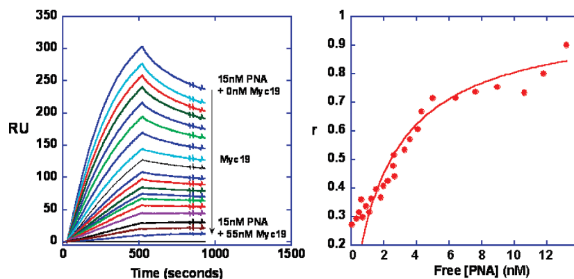
Figure 11. SPR competition experiment for measuring equilibrium constant for D-Ala-P eg2 + Myc19 hybridization in solution. All samples contained 15 nM PNA, 10 mM Tris HCl (pH 7), 0.1 mM Na 2 EDTA, and 100 mM KCl with varying concentrations of Myc19 . (Left) SPR data for individual samples. (Right) Binding isotherm where r values ( r = [\text{PNA bound}]/[\text{DNA total}] ) were calculated on the basis of the amount of free PNA available to hybridize to the SPR surface. Line corresponds to fit based on 1:1 binding equation.
